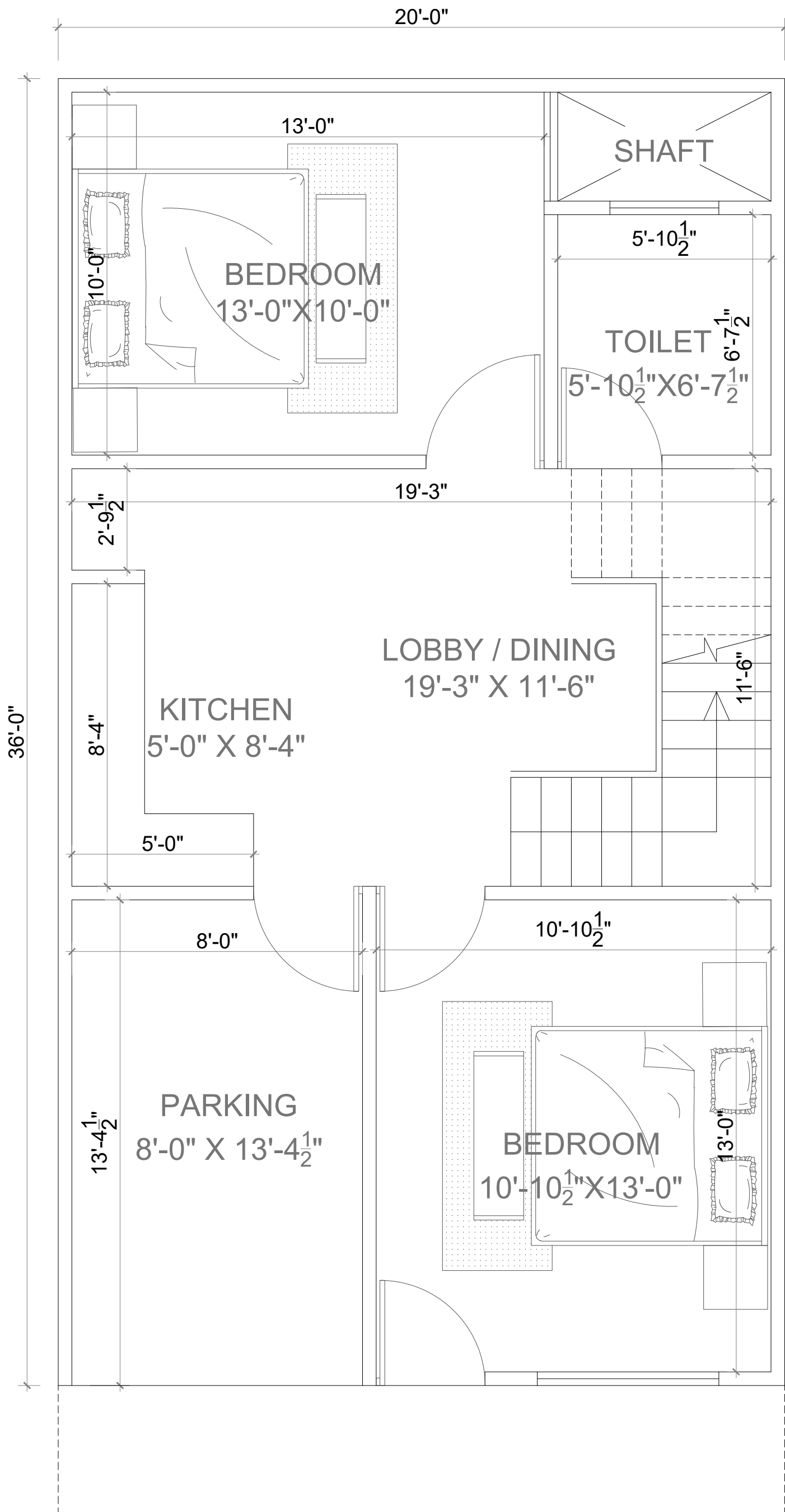
GROUND FLOOR PLAN TOTAL AREA = 720 SQFT = 80 SQYD
